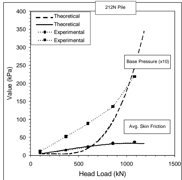
Figure 11. Comparative Results for the 212N Pile.
