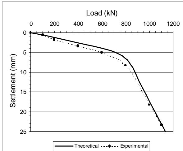
Figure 7. Load-Displacement Curve Obtained for the 212N Pile (after Cunha et al. 2002).
