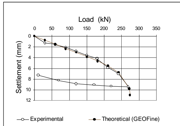
Figure 6. Load-Displacement Curve Obtained for the UnB Pile (modified after Mota 2003).
