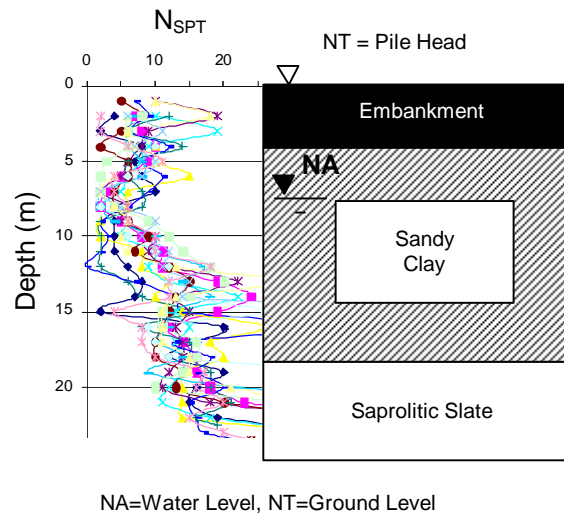
Figure 3. Geotechnical Profile of 212N Site.
