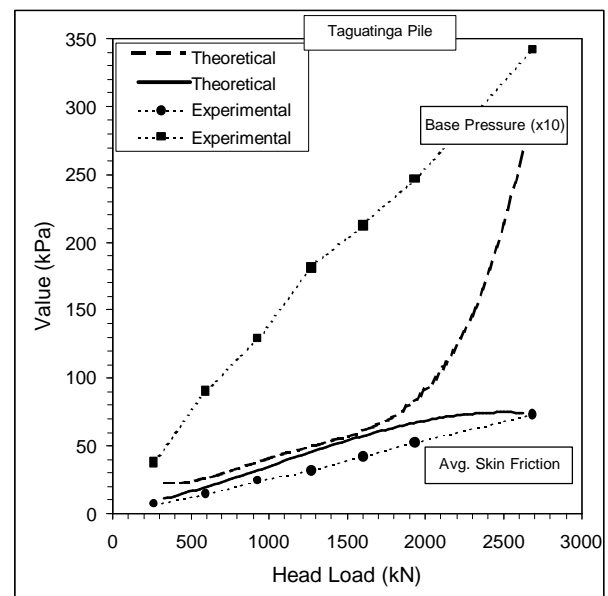
Figure 12. Comparative Results for the Taguatinga Pile.
