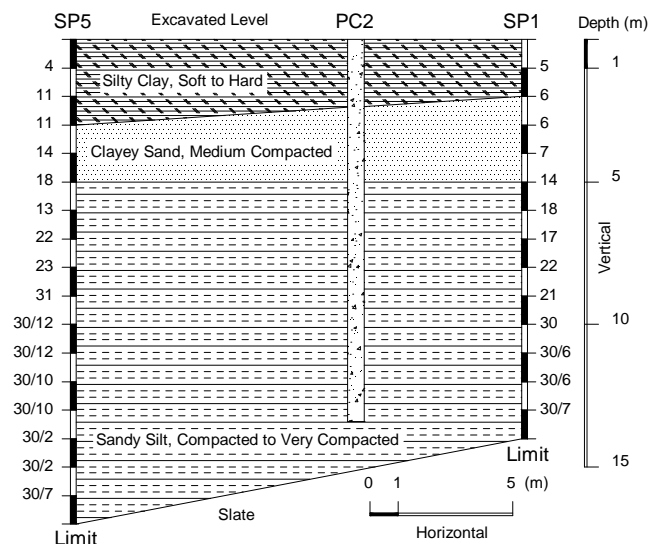
Figure 4. Geotechnical Profile of Taguatinga Site. (Cunha et al. 2003).
