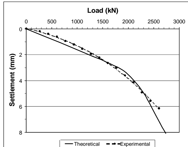
Figure 8. Load-Displacement Curve Obtained for the Taguatinga Pile.
