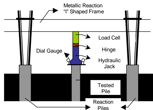
Figure 5. Schematic Drawing of the Field Load Testing System.
