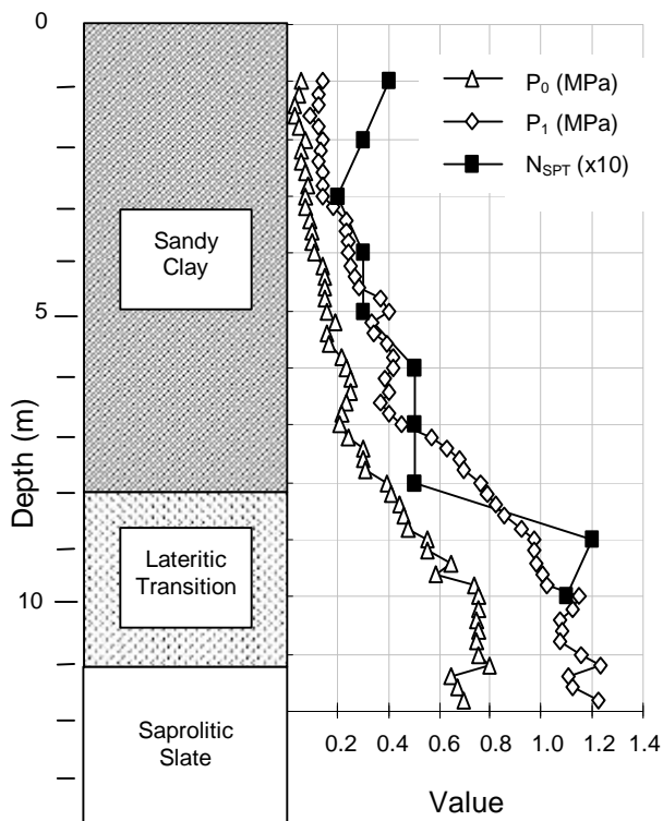
Figure 2. Geotechnical Profile of the UnB Site.
