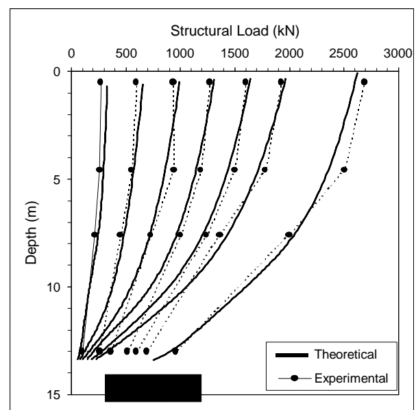
Figure 10. Load Transfer Curves - Taguatinga Pile.
